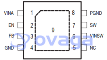
HSOP-8
